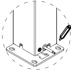
3.11、 Mark the drill holes on the concrete floor
