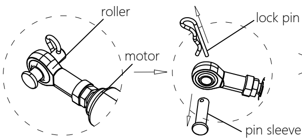
4.11-1、 take apart the pre-assembled lock pin and sleeve in advance
