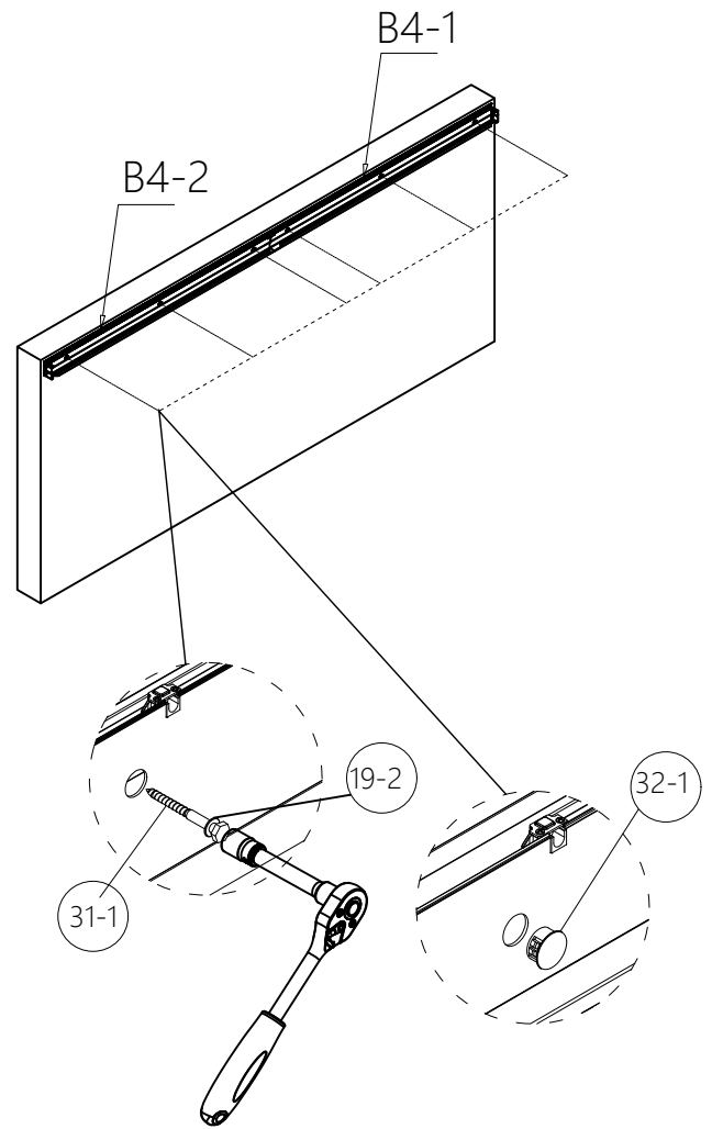
1.5、 use wrench to screw the beam B4-1 B4-2 on the wall
