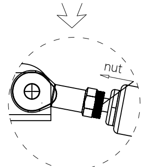
4.11-4、 screw the nuts to fasten the motor with driven louver blade
