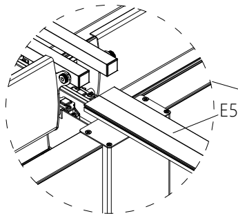
7.6 Insert the middle beam flashing
