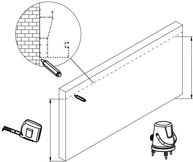
1.1、 Take use of gradienter to mark the wall mounted beam height and position
