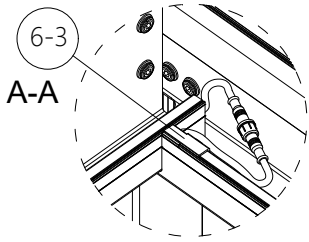
3.10、 Assemble the gutter decoration component
