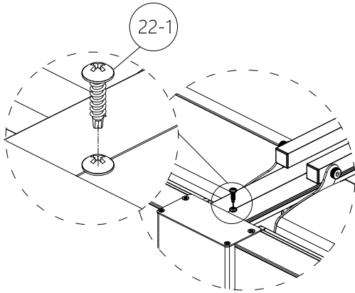
7.7 Screw the beam&gutter flashing.
