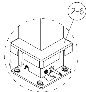
7.8 install the base plate covers
