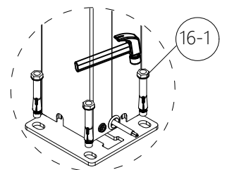
3.13、 Stuff the expansion bolts into concrete
